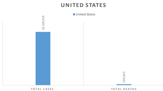
Figure 6: Actual country statistics [2].
