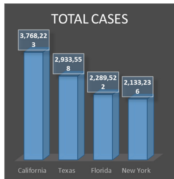
Figure 3: Comparison of actual total cases [2].
