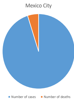
Figure 1: Actual Mexico City statistics [1].
