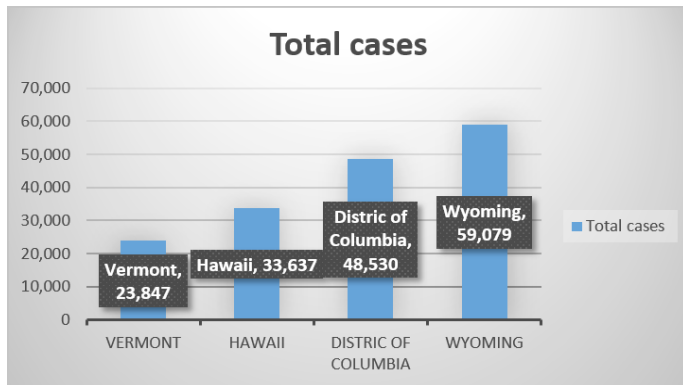
Figure 5: Comparison of actual total cases [2].
