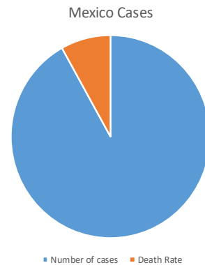
Figure 7: Actual country statistics.
